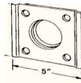
CT28938 Mounting Bracket & Snap Ring
