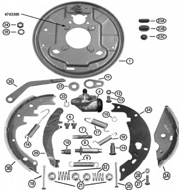
10" x 2 1/4" Free Backing w/ Parking Brake Diagram
